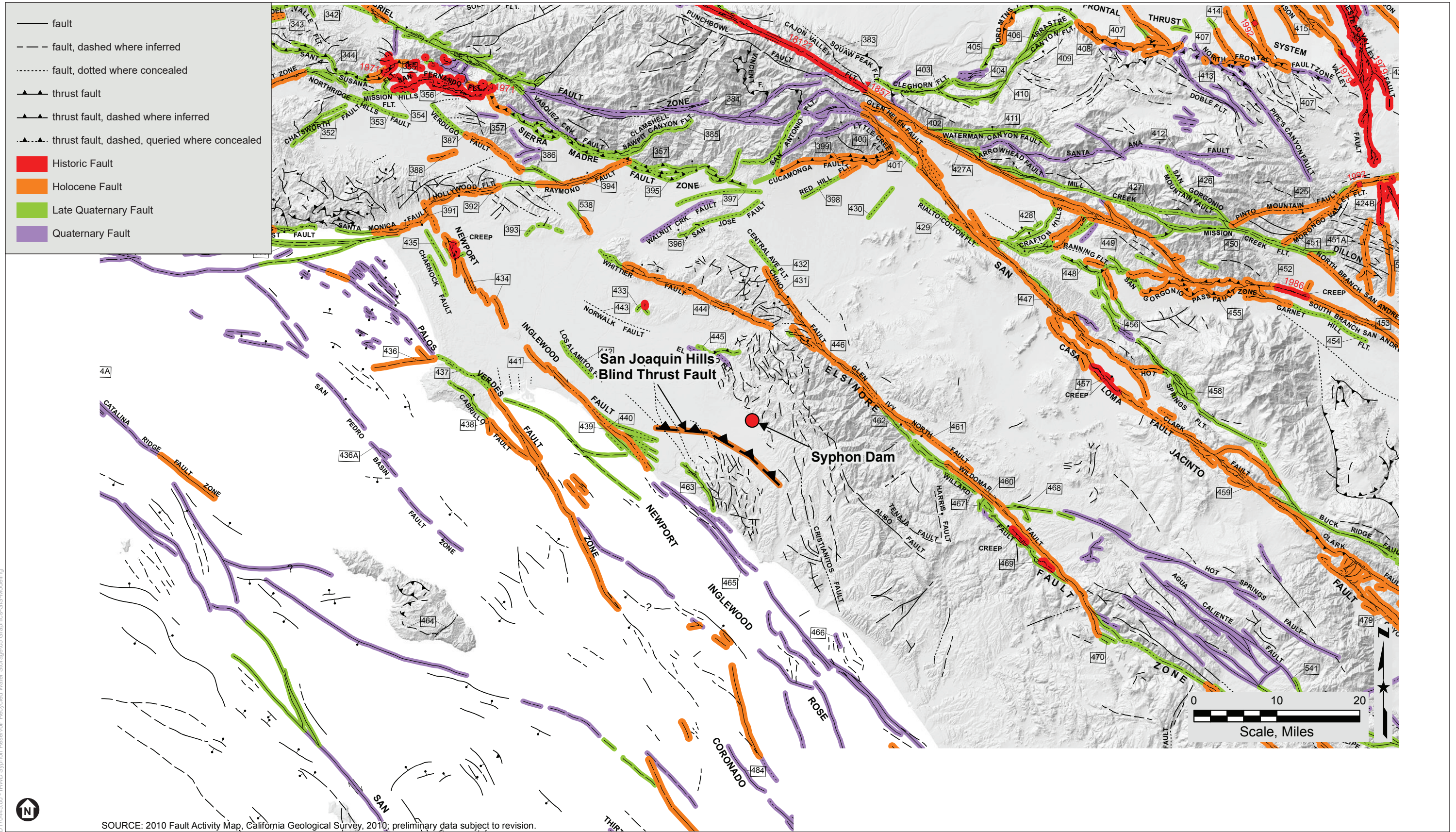
Figure 3.6-4 Regional Faults
