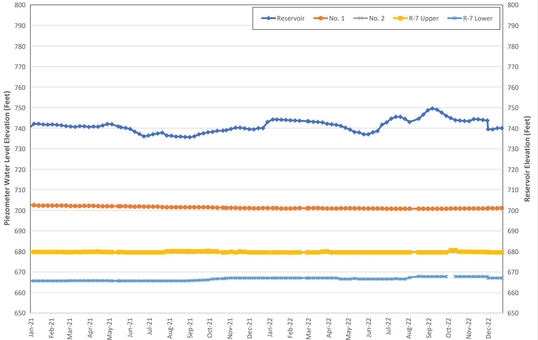
Figure 6 SANTIAGO CREEK DAM 2-YR OPEN WELL PIEZOMETER AND RESERVOIR WATER SURFACE ELEVATIONS PIEZOMETERS No. 1, No. 2, AND R-7 JANUARY 2021 THROUGH DECEMBER 2022
