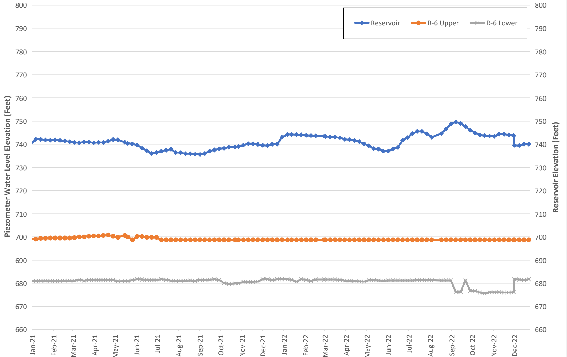
Figure 5 SANTIAGO CREEK DAM 2-YR OPEN WELL PIEZOMETER AND RESERVOIR WATER SURFACE ELEVATIONS PIEZOMETER R-6 JANUARY 2021 THROUGH DECEMBER 2022
