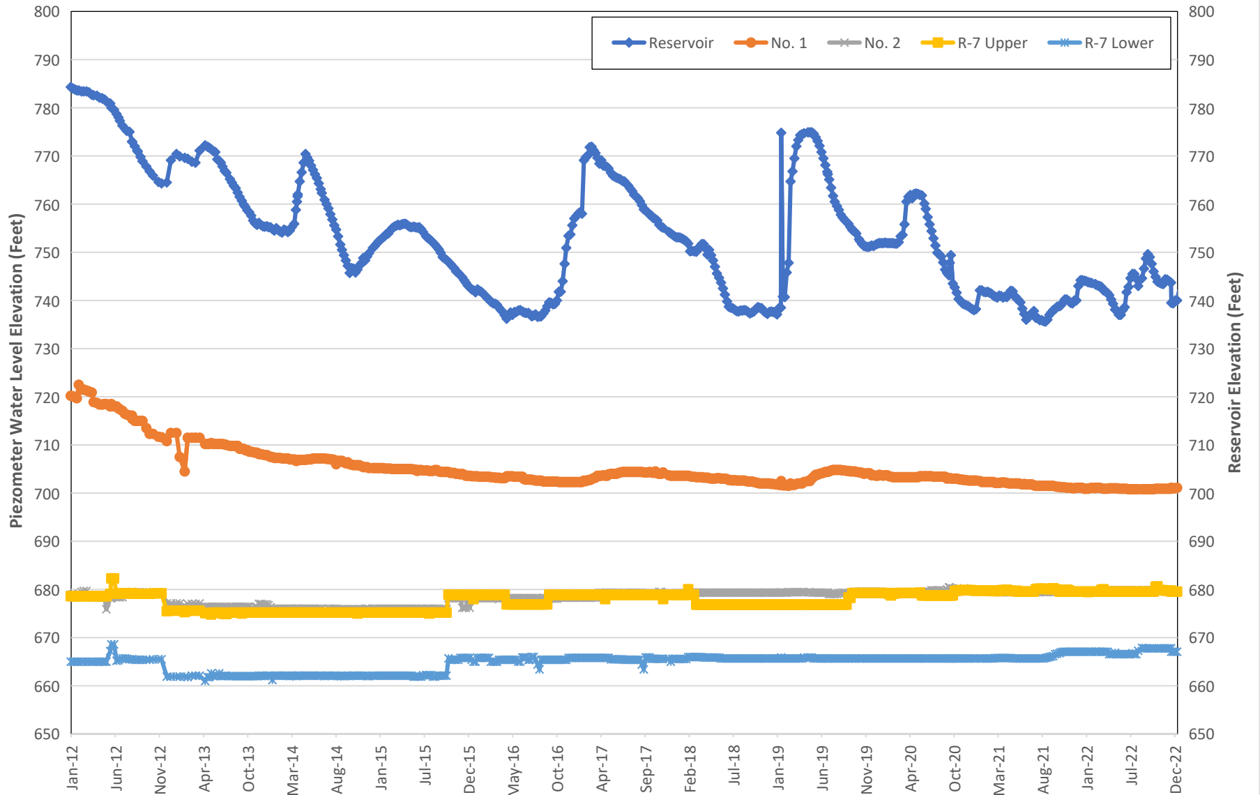
Figure 12 SANTIAGO CREEK DAM HISTORICAL PIEZOMETER AND RESERVOIR WATER SURFACE ELEVATIONS PIEZOMETERS No. 1, No. 2, AND R-7 JANUARY 2012 THROUGH DECEMBER 2022
