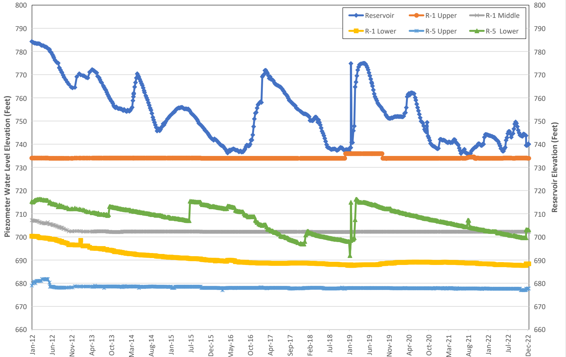
Figure 8 SANTIAGO CREEK DAM HISTORICAL PIEZOMETER AND RESERVOIR WATER SURFACE ELEVATIONS PIEZOMETERS R-1 AND R-5 JANUARY 2012 THROUGH DECEMBER 2022
