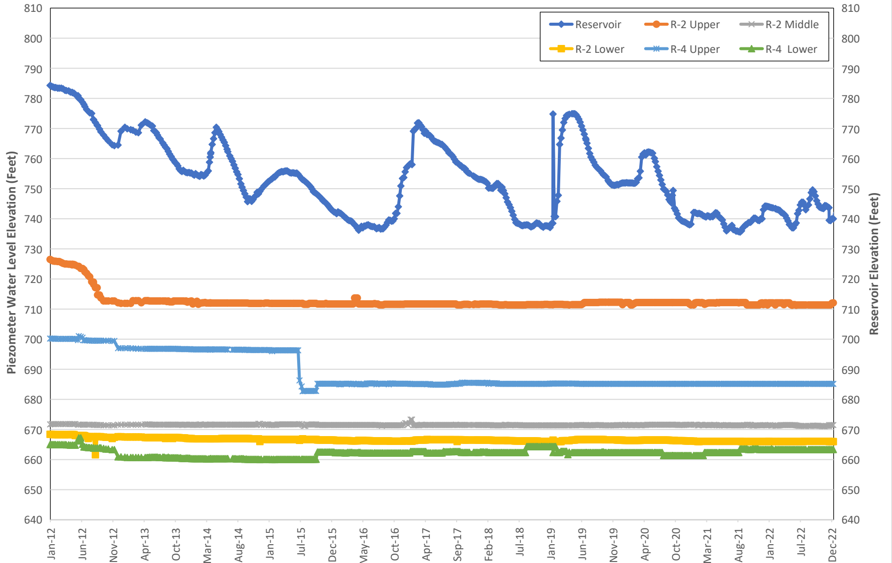
Figure 9 SANTIAGO CREEK DAM HISTORICAL PIEZOMETER AND RESERVOIR WATER SURFACE ELEVATIONS PIEZOMETERS R-2 AND R-4 JANUARY 2012 THROUGH DECEMBER 2022
