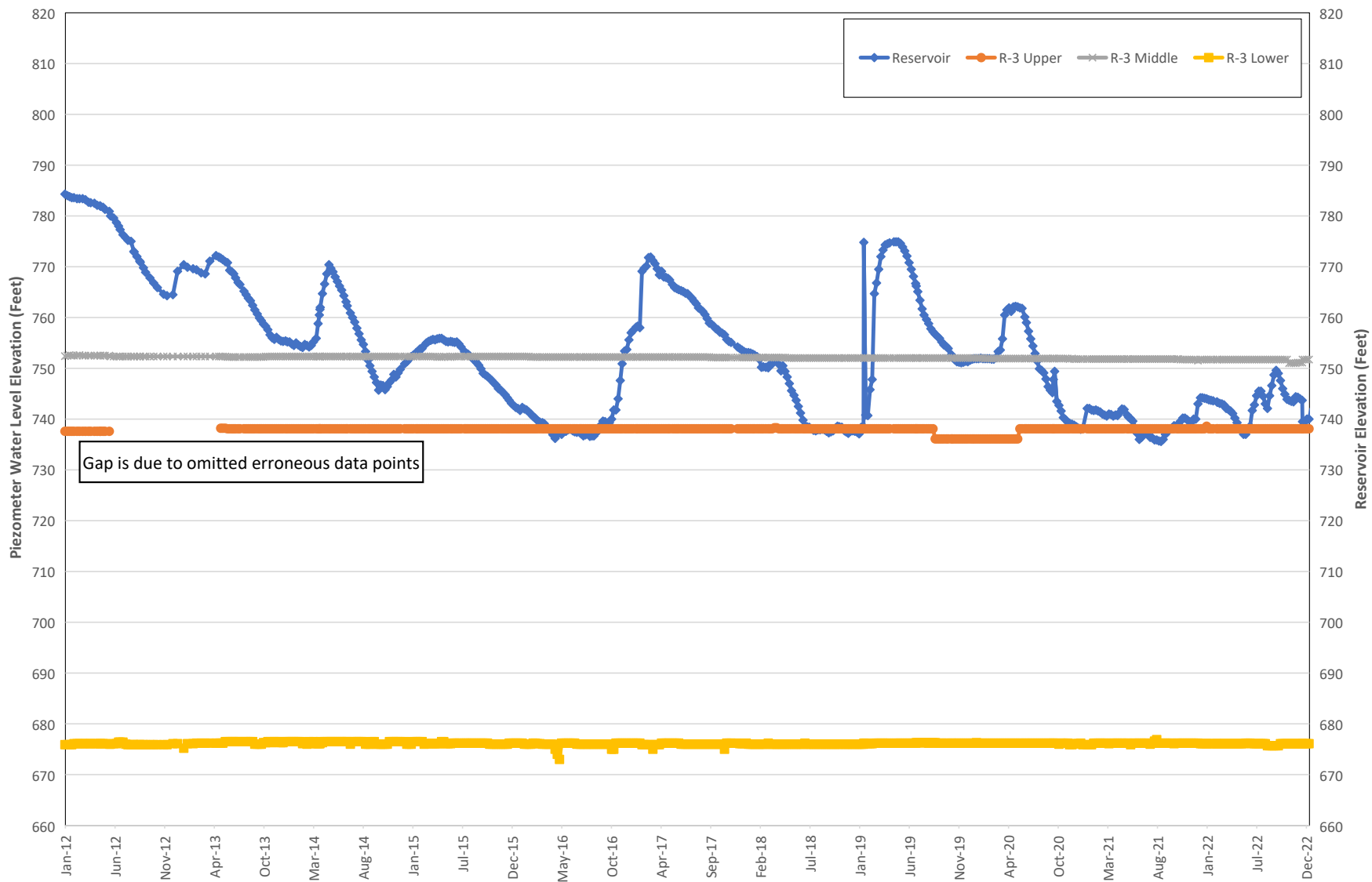
Figure 10 SANTIAGO CREEK DAM HISTORICAL PIEZOMETER AND RESERVOIR WATER SURFACE ELEVATIONS PIEZOMETER R-3 JANUARY 2012 THROUGH DECEMBER 2022
