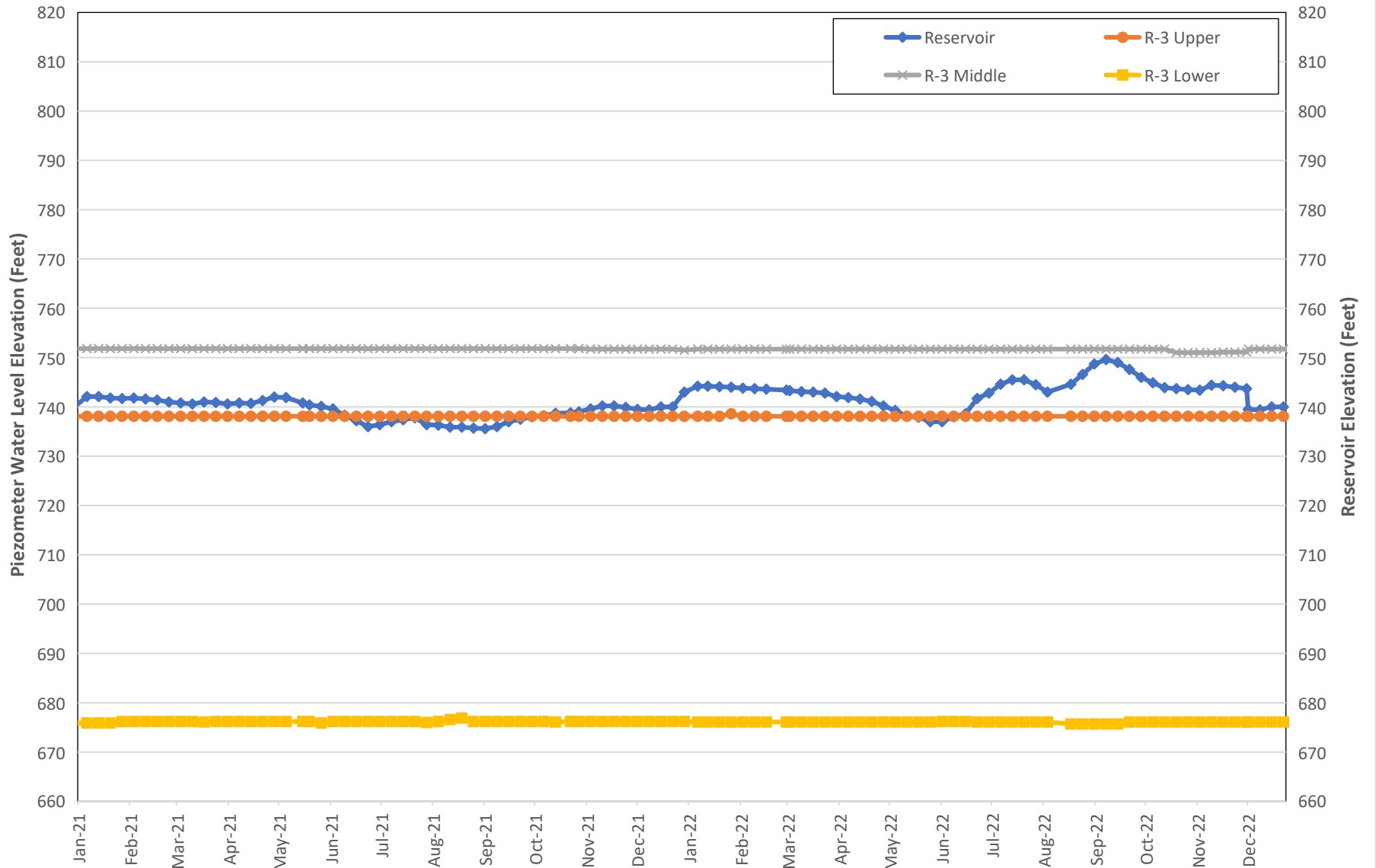
Figure 4 SANTIAGO CREEK DAM 2-YR OPEN WELL PIEZOMETER AND RESERVOIR WATER SURFACE ELEVATIONS PIEZOMETER R-3 JANUARY 2021 THROUGH DECEMBER 2022
