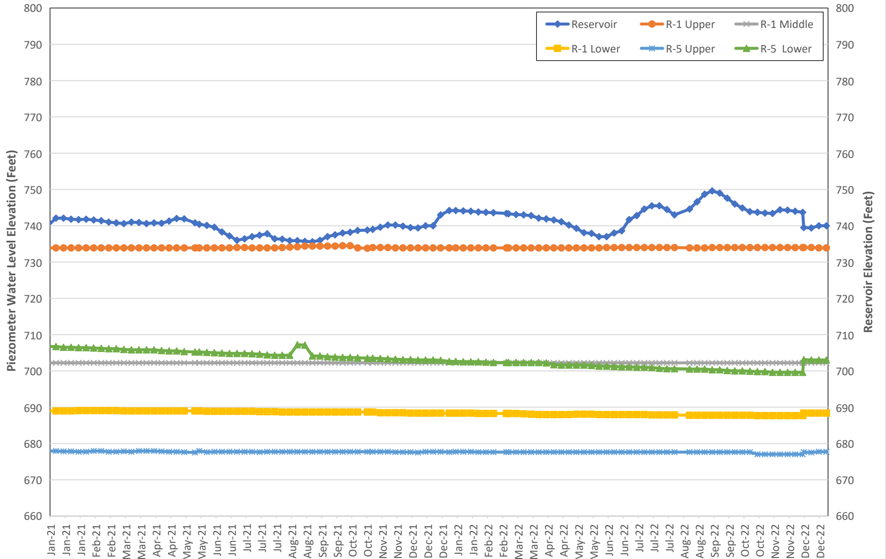
Figure 2 SANTIAGO CREEK DAM 2-YR OPEN WELL PIEZOMETER AND RESERVOIR WATER SURFACE ELEVATIONS PIEZOMETERS R-1 AND R-5 JANUARY 2021 THROUGH DECEMBER 2022
