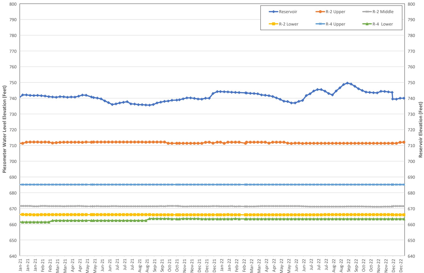
Figure 3 SANTIAGO CREEK DAM 2-YR OPEN WELL PIEZOMETER AND RESERVOIR WATER SURFACE ELEVATIONS PIEZOMETERS R-2 AND R-4 JANUARY 2021 THROUGH DECEMBER 2022
