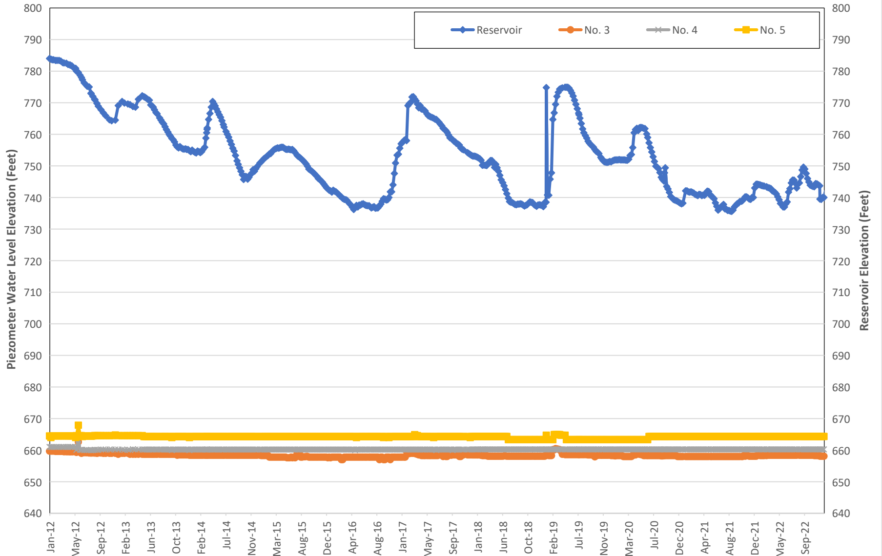
Figure 13 SANTIAGO CREEK DAM HISTORICAL PIEZOMETER AND RESERVOIR WATER SURFACE ELEVATIONS PIEZOMETERS No. 3, No. 4, No. 5 JANUARY 2012 THROUGH DECEMBER 2022
