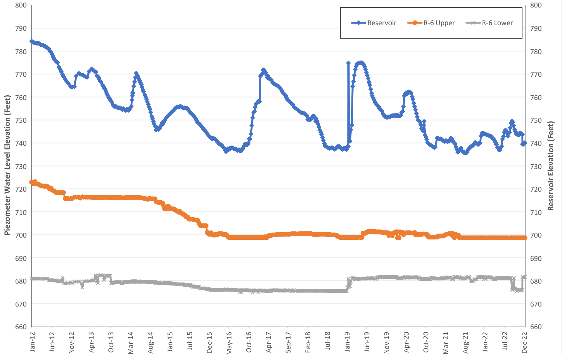
Figure 11 SANTIAGO CREEK DAM HISTORICAL PIEZOMETER AND RESERVOIR WATER SURFACE ELEVATIONS PIEZOMETER R-6 JANUARY 2012 THROUGH DECEMBER 2022
