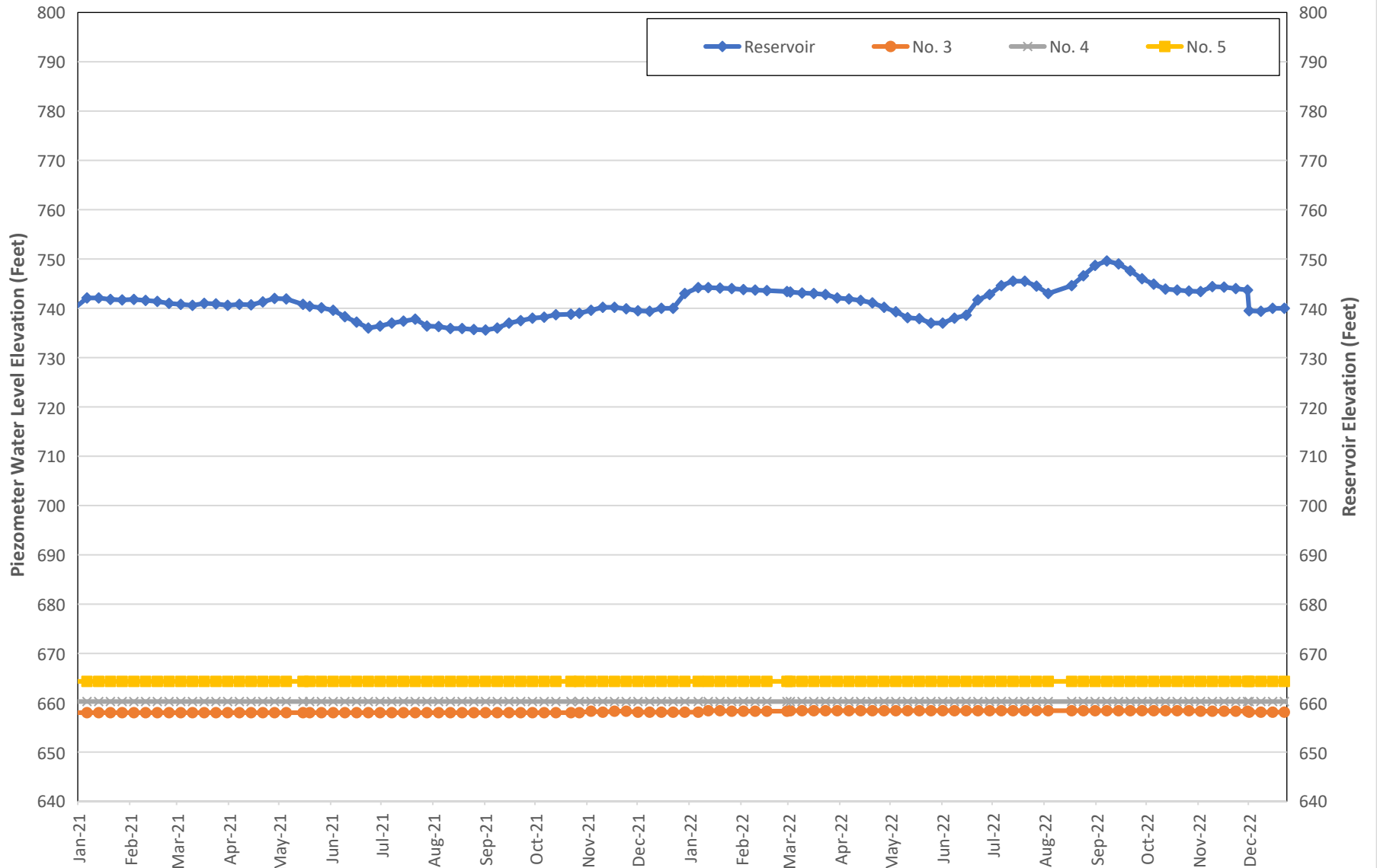
Figure 7 SANTIAGO CREEK DAM 2-YR OPEN WELL PIEZOMETER AND RESERVOIR WATER SURFACE ELEVATIONS PIEZOMETERS No. 3, No. 4, No. 5 JANUARY 2021 THROUGH DECEMBER 2022
